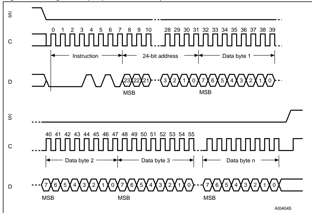
Figure 12. Page write (PW) instruction sequence
