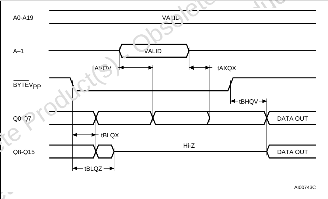
Figure 10. \overline{\text{BYTE}} Transition AC Waveforms
