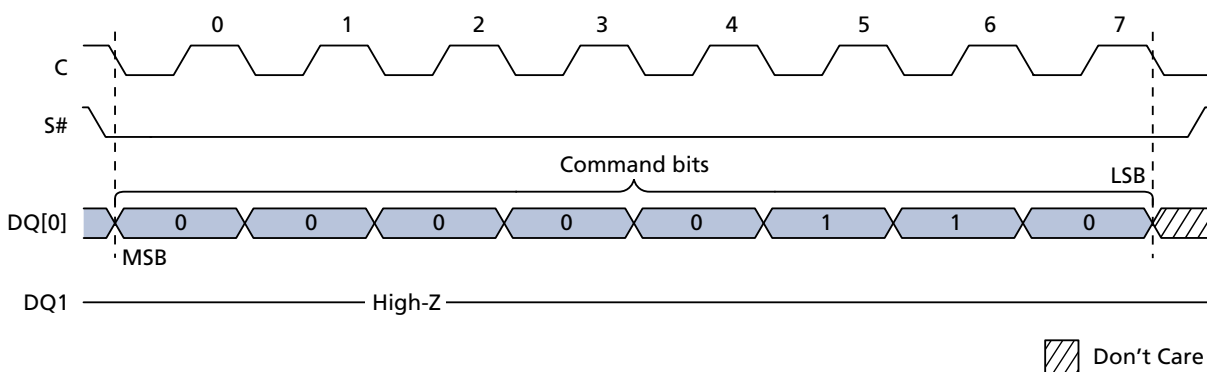
Figure 7: WRITE ENABLE Command Sequence
