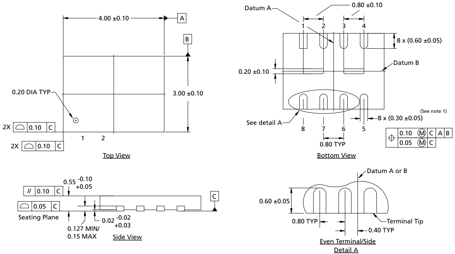
Figure 30: UFDFPN8 (MLP8) 4mm x 3mm
