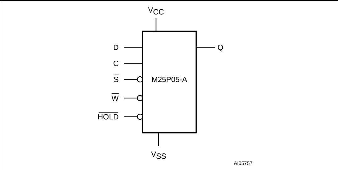
Figure 1. Logic diagram
