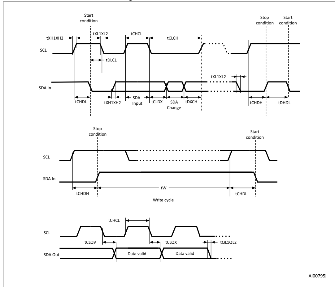
Figure 11. AC waveforms
