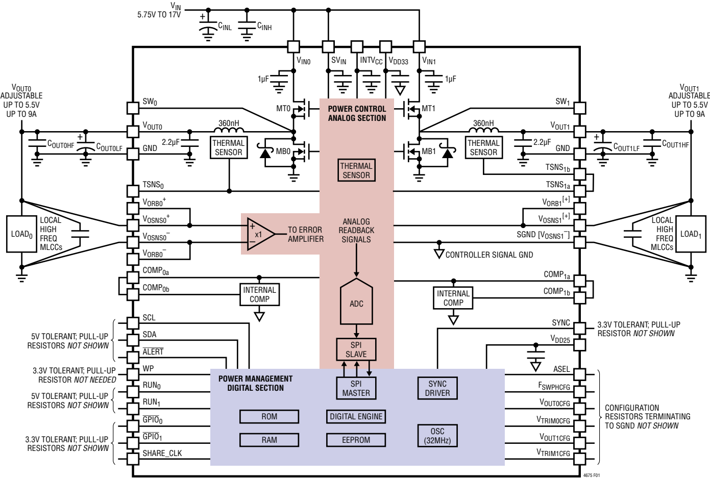
Figure 1. Simplified LTM4675 Block Diagram
