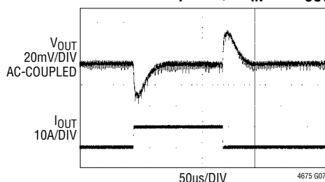
FIGURE 27 CIRCUIT AT 5\text{V}_{\text{IN}} . VOUT_COMMAND n SET TO 1.000V. 8A TO 18A LOAD STEP AT 10A/μs
