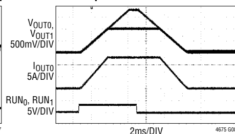
FIGURE 61 CIRCUIT AT 12\text{V}_{\text{IN}} . 112mΩ LOAD ON VOUT 0 . NO LOAD ON VOUT 1 . TON_RISE 0 = 3ms, TON_RISE 1 = 5.297ms, TOFF_DELAY 1 = 0ms, TOFF_DELAY 0 = 2.43ms, TOFF_FALL 1 = 5.328ms, TOFF_FALL 0 = 3ms, ON_OFF_CONFIG n = 0x1E
