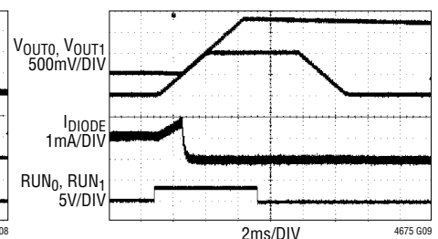
FIGURE 61 CIRCUIT AT 12\text{V}_{\text{IN}} . 112mΩ LOAD ON VOUT 0 . 500Ω ON VOUT 1 . VOUT 1 PRE-BIASED THROUGH A DIODE. TON_RISE 0 = 3ms, TON_RISE 1 = 5.297ms, TOFF_DELAY 1 = 0ms, TOFF_DELAY 0 = 2.43ms, TOFF_FALL 1 = 5.328ms, TOFF_FALL 0 = 3ms, ON_OFF_CONFIG 1 = 0x1F, ON_OFF_CONFIG 0 = 0x1E
