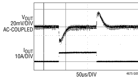
FIGURE 27 CIRCUIT AT 12\text{V}_{\text{IN}} . INTV CC PIN OPEN CIRCUIT AND VOUT_COMMAND n SET TO 1.000V. 8A TO 18A LOAD STEP AT 10A/μs
