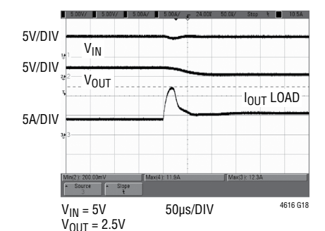
Short-Circuit Protection (2.5V Short, 4A Load)
