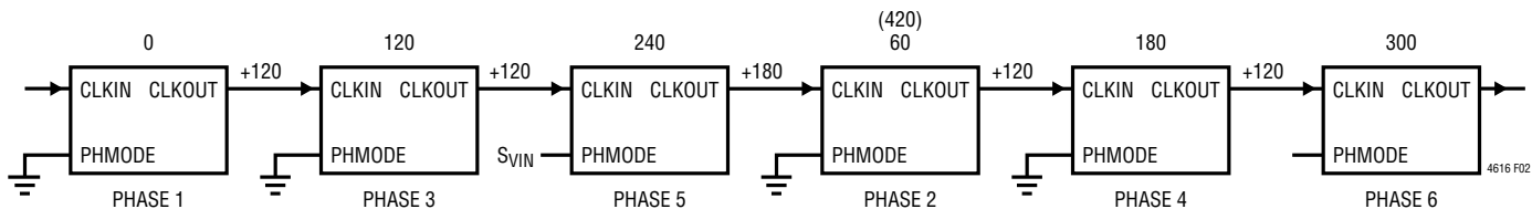
Figure 2. 6-Phase Operation
