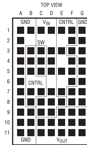
LGA PACKAGE 68-LEAD (15mm × 9mm × 2.82mm)
