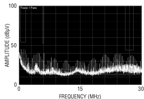
CISPR-25 CONDUCTED EMI MEASUREMENT WITH ADDITIONAL INPUT FILTER ( L = 240nH , C = 33µF ) V_{IN} = 13.5V , I_{OUT} = 8A
