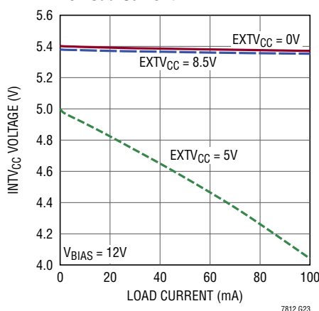
INTV CC and EXT CC vs Load Current
