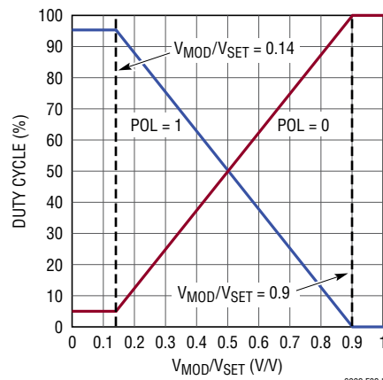
LTC6992-4
