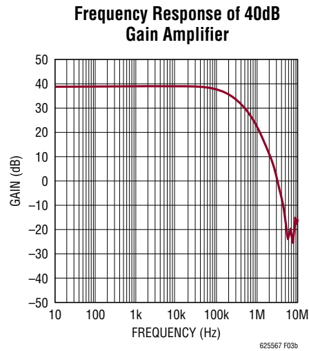
Figure 3. Gain of 100 Amplifier (3dB Bandwidth of 200kHz on 130 \mu A Supply Current)
