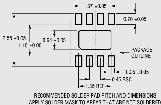
KC Package 8-Lead Plastic UTDFN (2mm × 2mm) (Reference LTC DWG # 05-08-1749 Rev 0)
