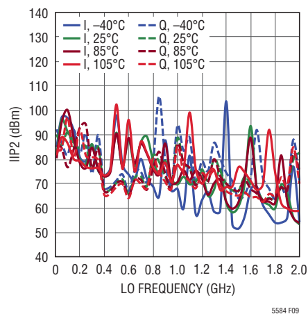
Figure 9. Broadband IIP2
