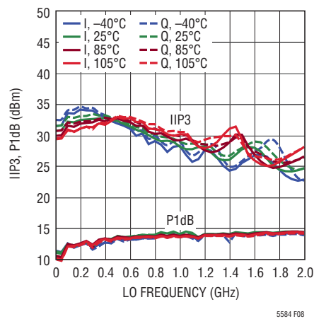
Figure 8. Broadband IIP3 and IP1dB
