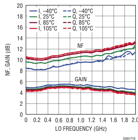
Figure 10. Broadband NF and Gain
