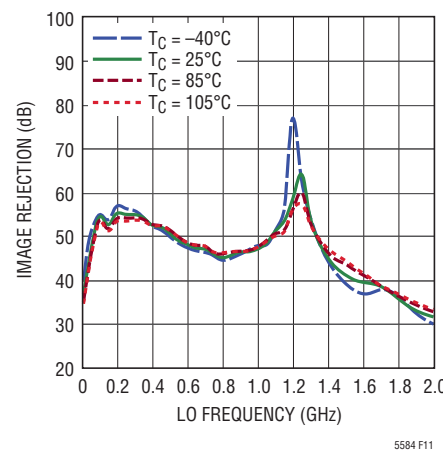
Figure 11. Broadband Image Rejection
