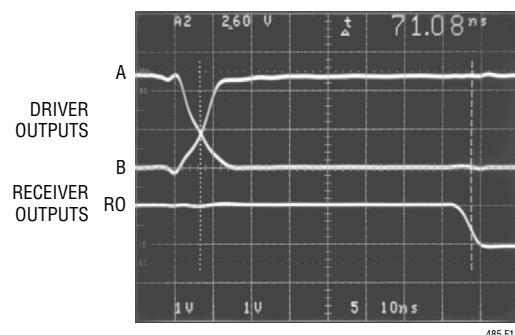
Figure 12. Receiver t_{PLH}
