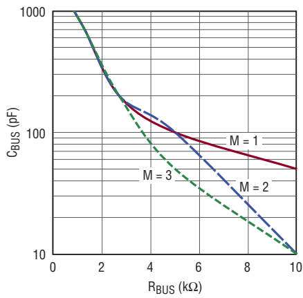
Figure 11. Recommended Maximum R_1 and C_{B1} Values for the LTC4313 Operating with Multiple LTC4300As in a 3.3V System
