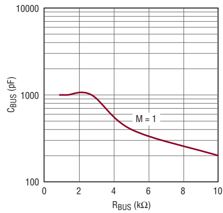
Figure 12. Recommended Maximum R_1 and C_{B1} Values for the LTC4313 Operating with Multiple LTC4307s in a 3.3V System
