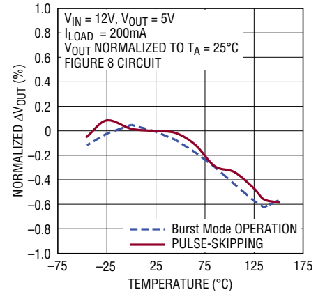
Output Regulation Over Temperature
