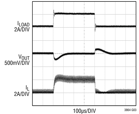
V_{IN} = 12\text{V} V_{OUT} = 5\text{V} TRANSIENT = 100mA TO 2A FIGURE 8 CIRCUIT
