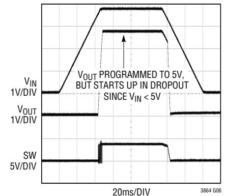
V_{IN} = 0\text{V} TO 3.8V THEN BACK TO 0V I_{LOAD} = 100\text{mA} FIGURE 8 CIRCUIT
