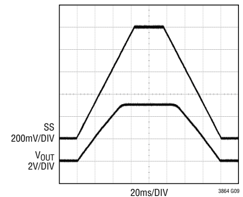
V_{IN} = 12\text{V} , V_{OUT} = 5\text{V} I_{LOAD} = 100\text{mA} FIGURE 8 CIRCUIT
