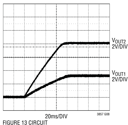
Soft Start-Up
