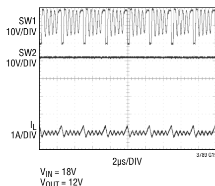
Pulse-Skipping Mode
