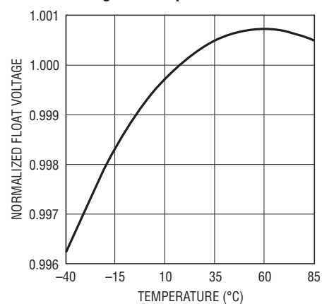
Normalized Battery Charger Float Voltage vs Temperature
