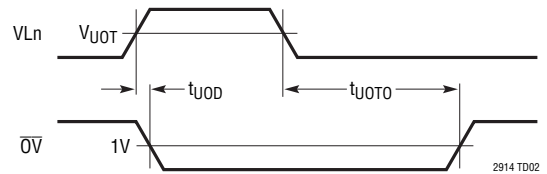
VLn Monitor Timing
