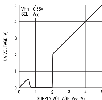
\overline{\text{UV}} Output Voltage vs V_{CC}
