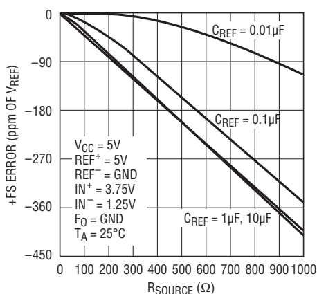
Figure 27. +FS Error vs R_{SOURCE} at REF^+ and REF^- (Large C_{REF} )
