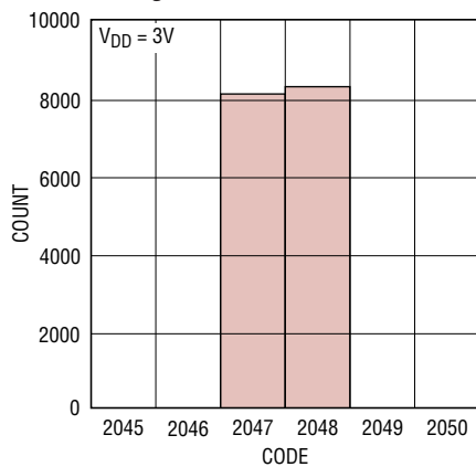
Histogram for 16384 Conversions
