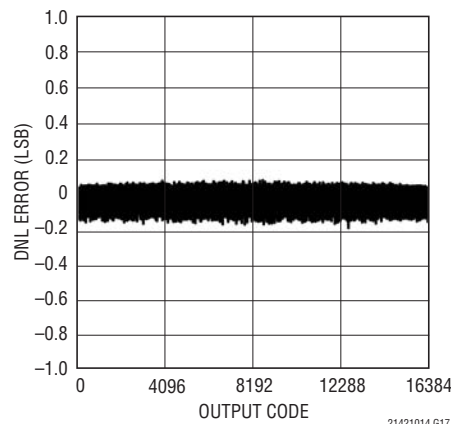
LTC2141-14: Differential Nonlinearity (DNL)
