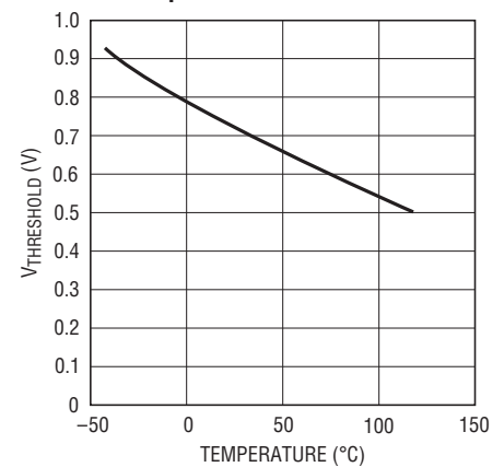
\overline{\text{SHDN}} Pin Threshold Voltage vs Temperature
