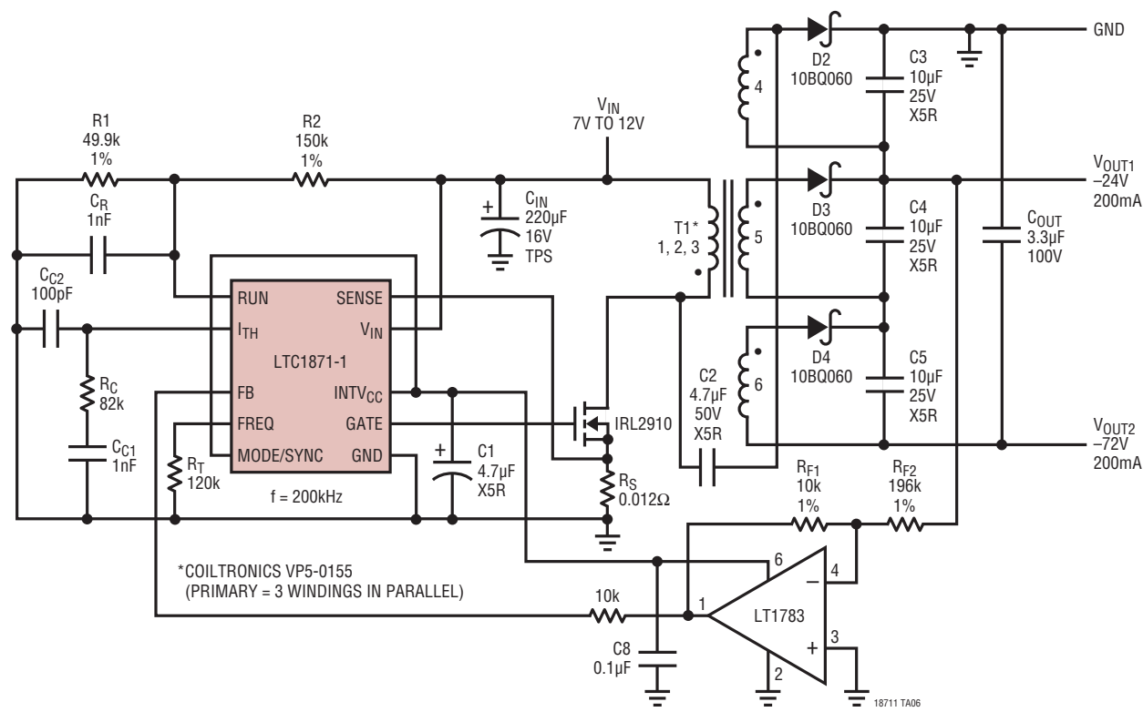
High Power SLIC Supply with Undervoltage Lockout (Also See the LTC3704 Data Sheet)
