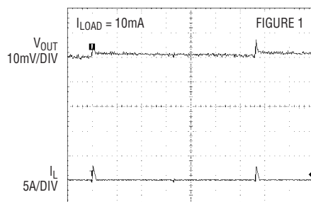
V_{OUT}(RIPPLE) (Synchronized)
