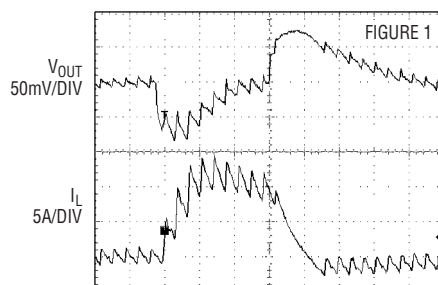
Load Step (Continuous Mode)
