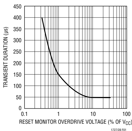
Figure 1. Transient Duration vs Comparator Overdrive
