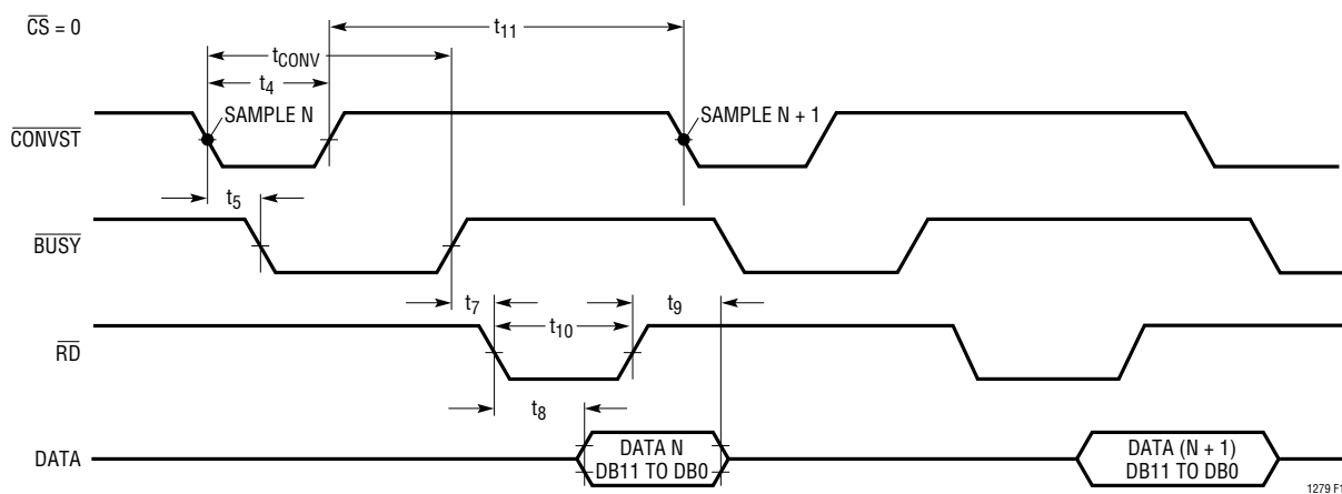
Figure 14. Mode 2. \overline{\text{CONVST}} Starts a Conversion. Data is Read by \overline{\text{RD}}
