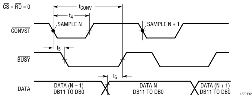
Figure 12. Mode 1a. \overline{CONVST} Starts a Conversion. Data Outputs Always Enabled. ( \overline{CONVST} = narrow pulse)
