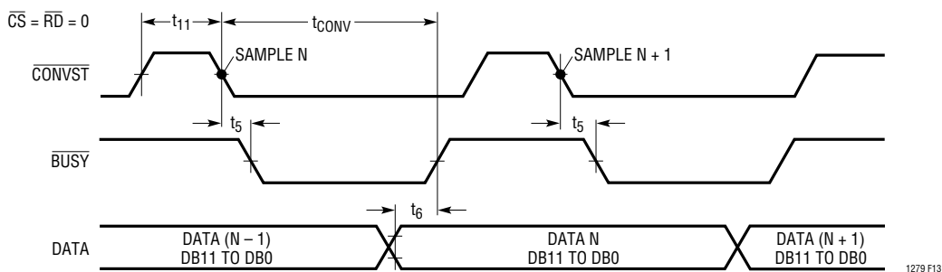
Figure 13. Mode 1b. \overline{\text{CONVST}} Starts a Conversion. Data Outputs Always Enabled. ( \overline{\text{CONVST}} = \text{Pulse} )
