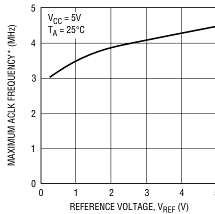
Maximum Conversion Clock Rate vs Reference Voltage
