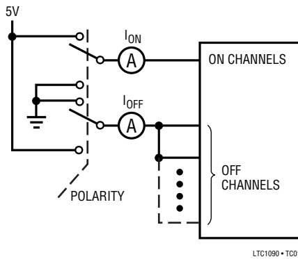
On and Off Channel Leakage Current
