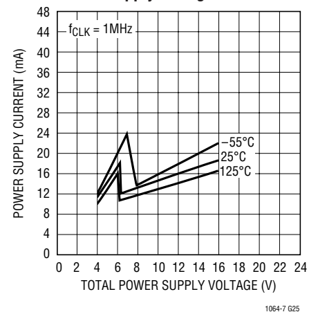
Power Supply Current vs Power Supply Voltage
