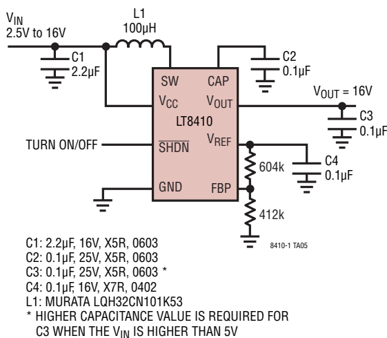
Figure 4. 16V Output Converter with Wide Input Voltage
