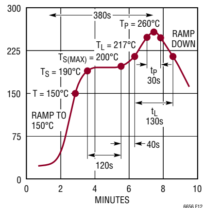
Figure 12. Lead Free Reflow Profile Due to IR Reflow
