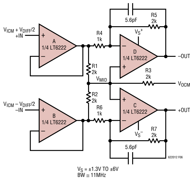
Figure 6. Buffered Gain of 2 Differential-In/Differential-Out Amplifier
