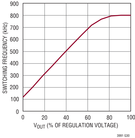
LT3991-X Frequency Foldback
