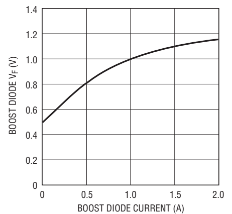
Boost Diode
