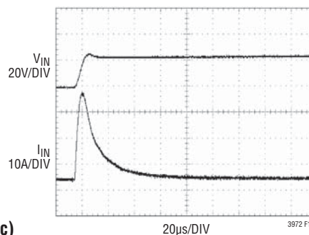
Figure 10. A Well Chosen Input Network Prevents Input Voltage Overshoot and Ensures Reliable Operation when the LT3972 is Connected to a Live Supply
