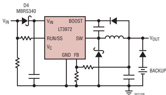
Figure 8. Diode D4 Prevents a Shorted Input from Discharging a Backup Battery Tied to the Output. It Also Protects the Circuit from a Reversed Input. The LT3972 Runs Only When the Input is Present
