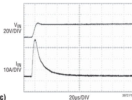
Figure 10. A Well Chosen Input Network Prevents Input Voltage Overshoot and Ensures Reliable Operation when the LT3972 is Connected to a Live Supply
