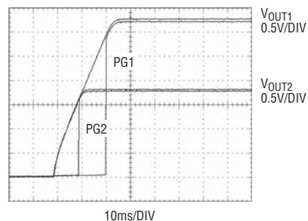
Absolute Start-Up
