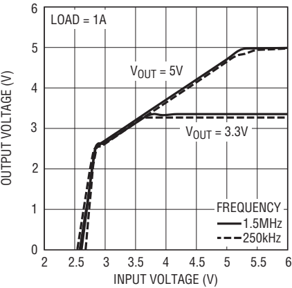
Dropout Operation
