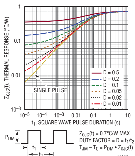
Figure 11. FQB34N20L Transient Thermal Response
