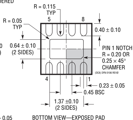
BOTTOM VIEW—EXPOSED PAD
