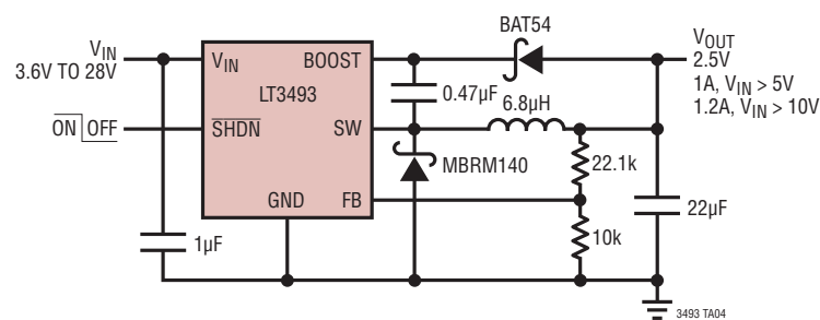
2.5V Step-Down Converter
