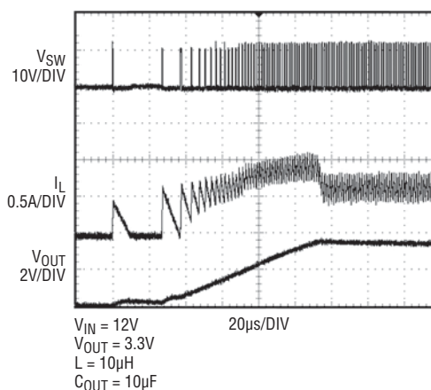
Figure 7. To Soft-Start the LT3493, Add a Resistor and Capacitor to the SHDN Pin. V IN = 12V, V OUT = 3.3V, C OUT = 10µF, R LOAD = 5Ω
