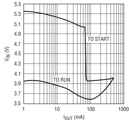
Typical Minimum Input Voltage ( V_{\text{OUT}} = 3.3\text{V} )
