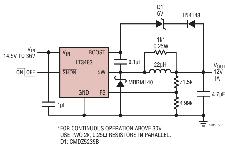
12V Step-Down Converter
