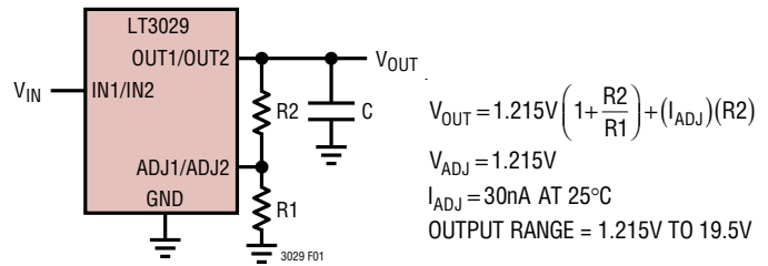
Figure 1. Adjustable Operation
