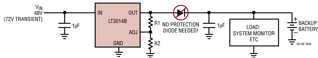
LT3014B Telecom Application
