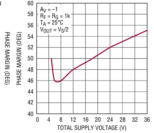
Phase Margin vs Supply Voltage
