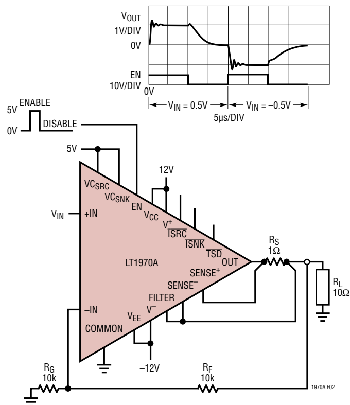
Figure 2. Using the ENABLE pin
