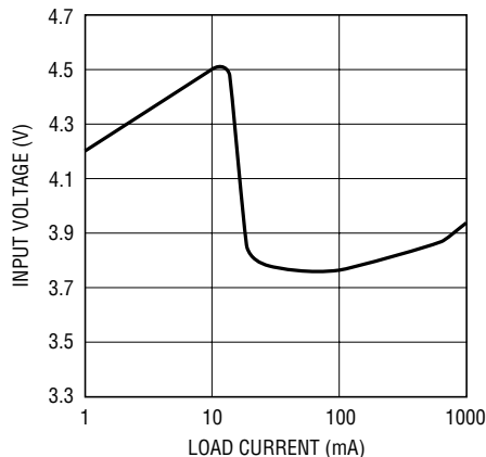
Minimum Input Voltage with 3.3V Output
