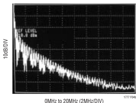
(b) LT1777 with L_{\text{SENSE}} = 0\mu\text{H}
