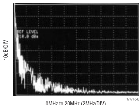
(c) LT1777 with L_{\text{SENSE}} = 2.2\mu\text{H}
