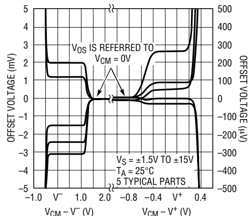
Offset Voltage Shift vs Common Mode
