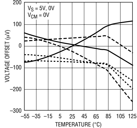
VOS vs Temperature of Representative Units
