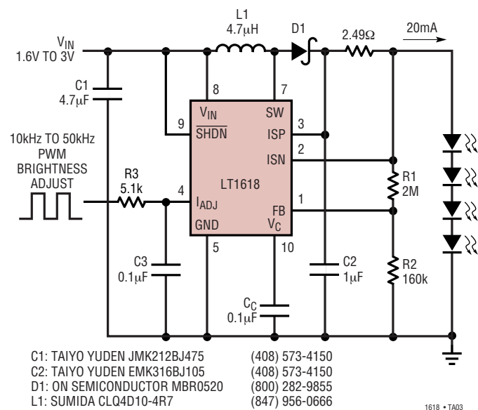
2-Cell White LED Driver
