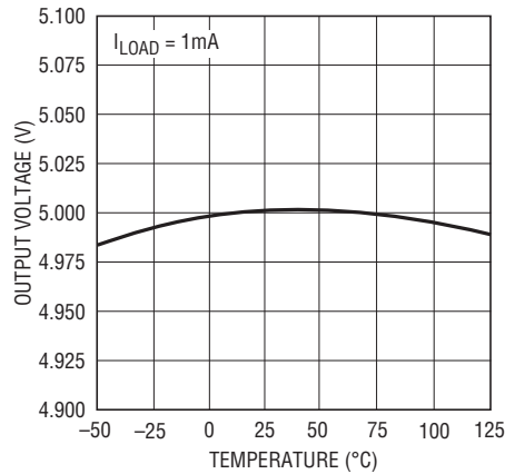
LT1129-5 Output Voltage
