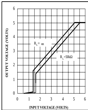
Dropout Characteristics
