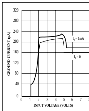
Ground Current
