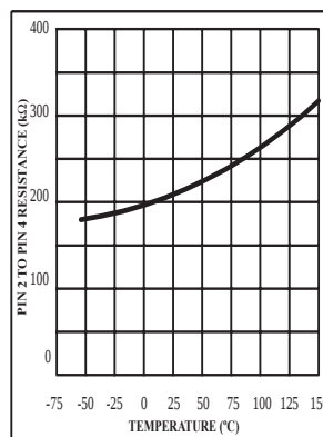
LP2951 Divider Resistance
