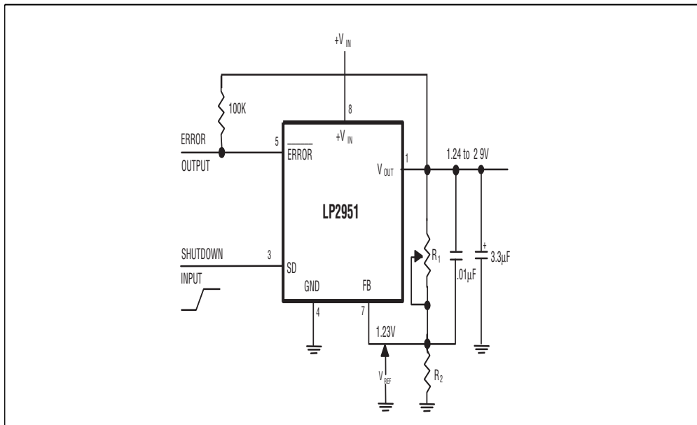
Figure 2. Adjustable Regulator
