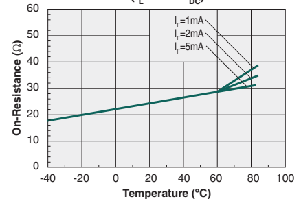
Typical On-Resistance vs. Temperature ( I_L = 70\text{mA}_{\text{DC}} )
