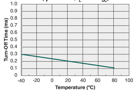
Typical Turn-Off Time vs. Temperature ( I_F = 0.25\text{mA} , I_L = 70\text{mA}_{\text{DC}} )
